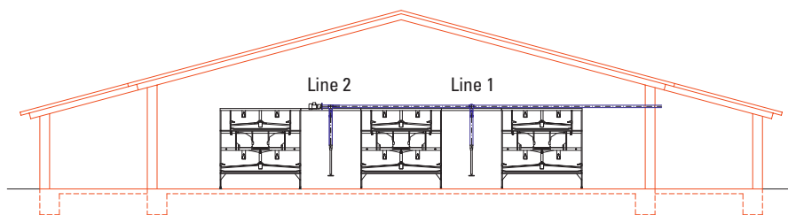
Cross section of the house: PickPuck with automatic filling
