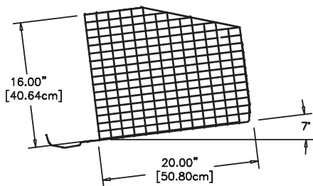
CAGE PARTITION (TOP TIER)
